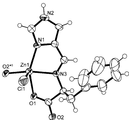
Figure 7. ORTEP drawing of [ZnClHL H ] ( 6 ) with the selected atom numbering scheme at 296 K, where the atom ellipsoids are 50% probability level.
