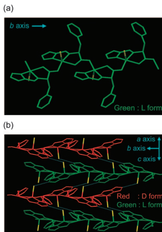
Figure 6. (a) Homochiral 1D chain structure of 4b constructed from intermolecular Cu–O *5 coordination bonds (* 5 represents the symmetry operation; -x, -1/2 + y, 3/2 - z ). (b) The heterochiral 2D network structure is constructed by interchain imidazole–Br − hydrogen bonds.
