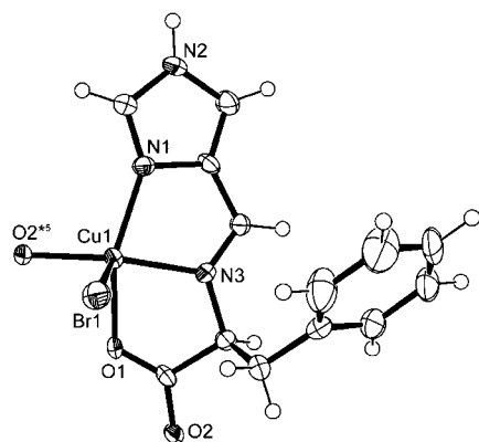
Figure 5. ORTEP drawing of [CuBrHL H ] ( 4b ) with the atom-numbering scheme at 180 K, where the thermal ellipsoids are presented at 50% probability level.
