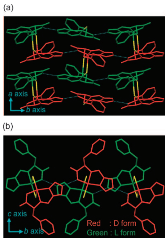
Figure 2. Heterochiral 2D network structure of [CuCIHL H ] (1), where red- and green-colored molecules represent two enantiomers consisting of D- and L-phenylalanine moieties, respectively. The homochiral chain is constructed by intermolecular imidazole-carboxylate hydrogen bonds (blue dots). The adjacent chains with opposite chiralities are linked by interchain Cu-Cl *2 coordination bond (yellow, *2 represents a symmetry operation of -x, -y, 2 - z ). (a) Side view of the 2D structure and (b) top view of the 2D structure.
