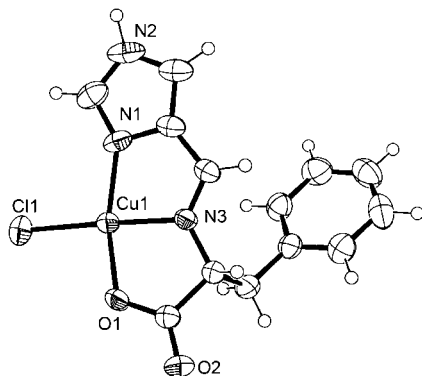
Figure 1. ORTEP drawing of [CuCIHL H ] ( 1 ) with the selected numbering scheme at 296 K, where the thermal ellipsoids are represented at 50% probability level.
