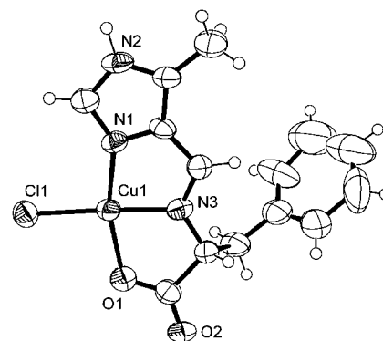
Figure 3. ORTEP drawing of [CuCIHL 5-Me ]·MeOH ( 3 ) with the selected atom-numbering scheme at 296 K, where the atom ellipsoids are 50% probability level.
