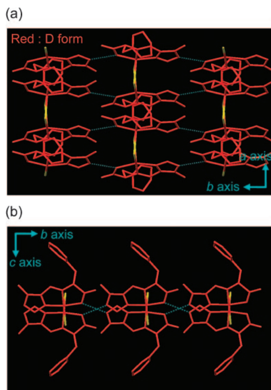
Figure 4. Homochiral 2D network structure of [CuCIHL 5-Me ]·MeOH ( 3 ), where the red-colored molecule represents one enantiomer consisting of the D-phenylalanine moiety. The homochiral chain is constructed by intrachain imidazole-carboxylate hydrogen bonds (blue dots). Adjacent chains with the same chirality are linked by the interchain coordination bond (yellow). (a) Side view of the 2D structure and (b) top view showing the stacking manner of the two adjacent chains.
