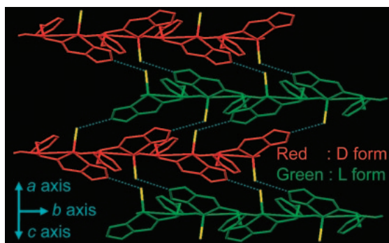
Figure 8. Homochiral 1D chain structure of 6 constructed by Zn–O *5 coordination bond and racemic 2D network structure. The heterochiral 2D network structure is constructed by interchain imidazole–Cl – hydrogen bonds.
