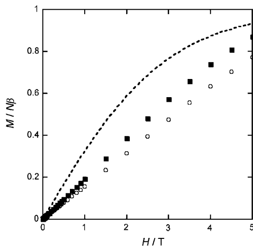
Figure 9. Field dependence of the magnetization of M at 2 K as a function of the applied magnetic field H for 3 (○) and 4b (■). The broken dotted line represents the theoretical curves for the Brillouin functions for Cu II ion S = 1/2 and g = 2.00 .
